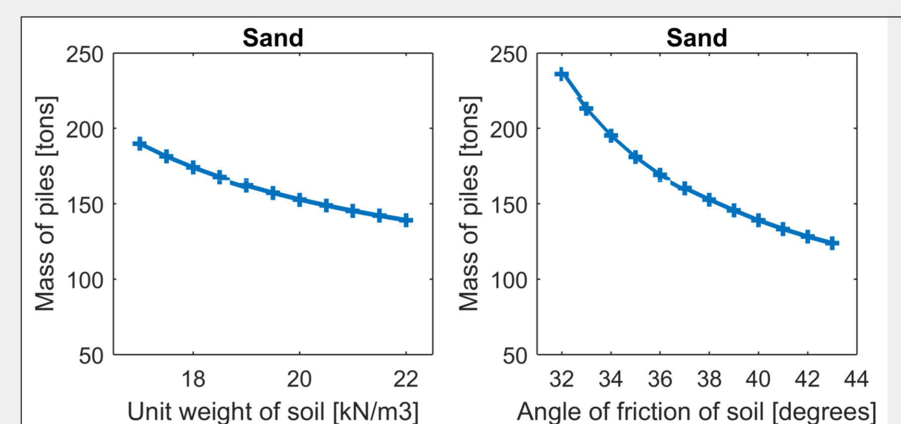
Figure 6: Result of parameter study for piles in sand. Both soil weight and angle of friction have a large influence on the pile design.
