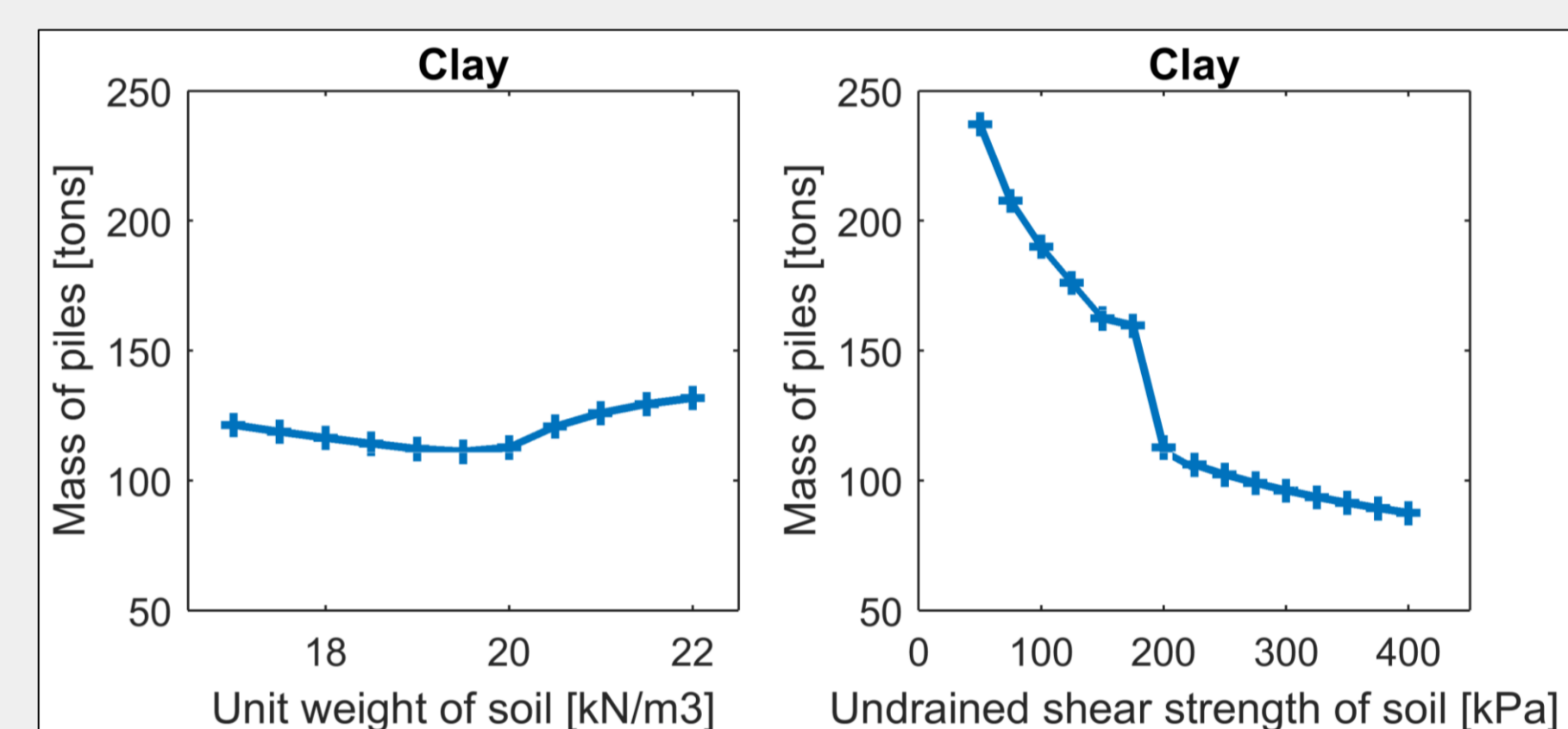
Figure 5: Result of parameter study for piles in clay. The shear strength has a large influence on the pile design.
